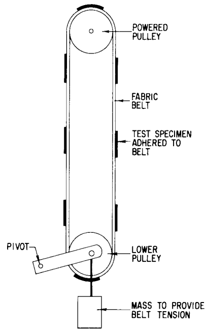
FIG. 3 Schematic Diagram of Method B Tester
