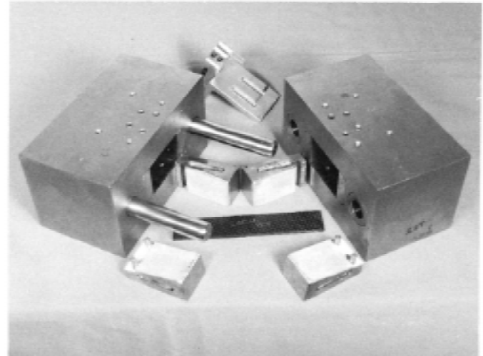
FIG. 7 Photograph of Compression Test Fixture
