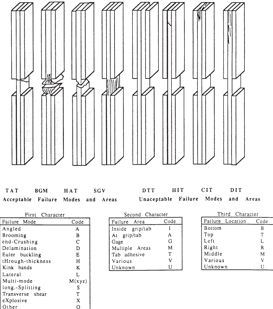
FIG. 9 Compression Test Specimen Three-Part Failure Identification Codes and Overall Specimen Failure Schematics
