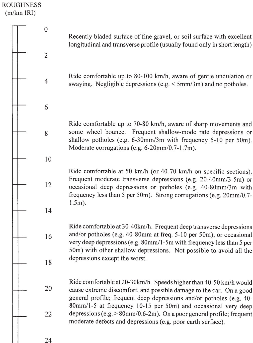
FIG. 2 Road Roughness Estimation Scale for Unpaved Roads with Gravel or Earth Surfaces
