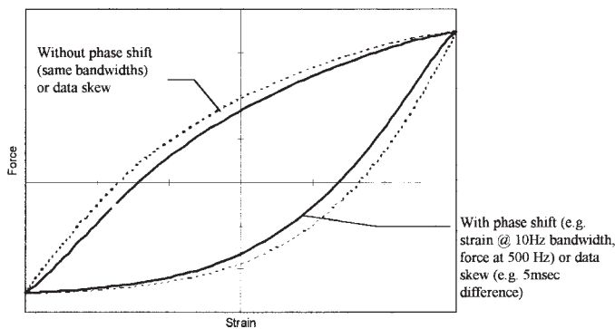
FIG. A1.13 Effect on Hysteresis Loop of Different Bandwidths or of Data Skew
