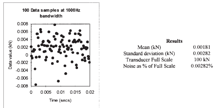
FIG. A1.11 Measuring System Noise Level
