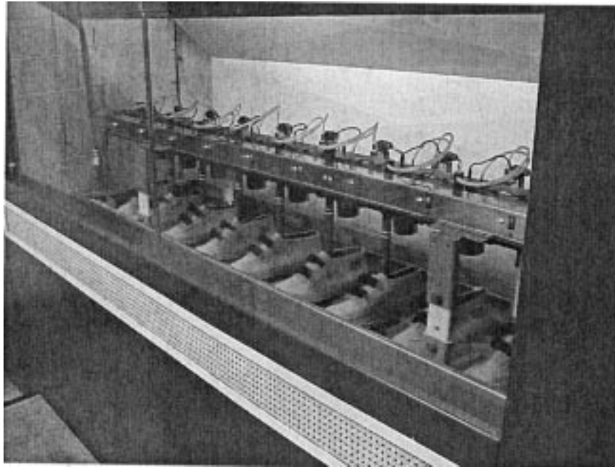
FIG. 1 Typical Test Arrangement for Dielectric Test of Rubbers Using Water Electrodes
