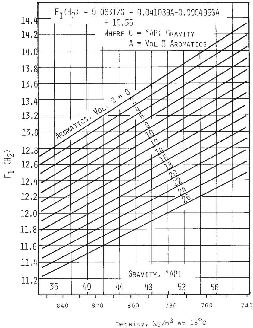
FIG. 1 Nomogram for Determining F_1(H_2)
